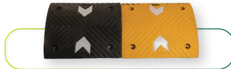
ARROW RUBBER SPEED BREAKER 75MM-2PC SIZE - 100 X 45 X 7.5 CM CODE - LSI - RHE -75MM-DR
