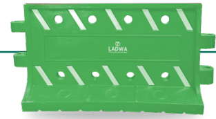
HEAVY DUTY ROAD BARRICADE SIZE - 2000 X 560 X 1000MM LSI-15.50KG-BARRICADE-MESH-GREEN
